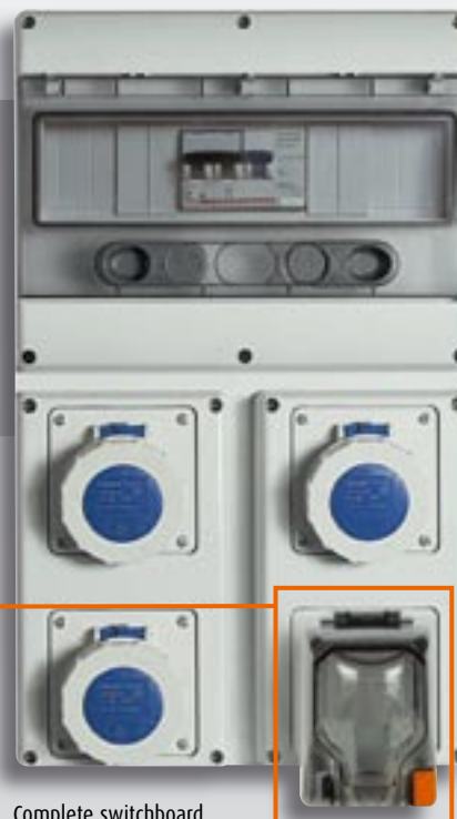
Complete switchboard
