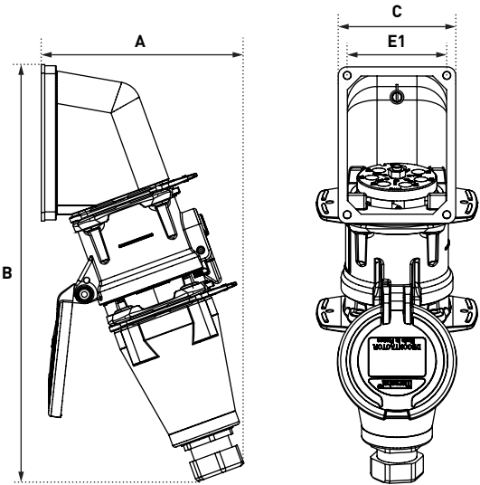
PLUG ON 70° INCLINED SOCKET-OUTLET
